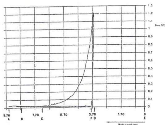
Figure 2 Diagram of pressure displacement plot in the energy analysis with 0.5% magnesium stearate.
