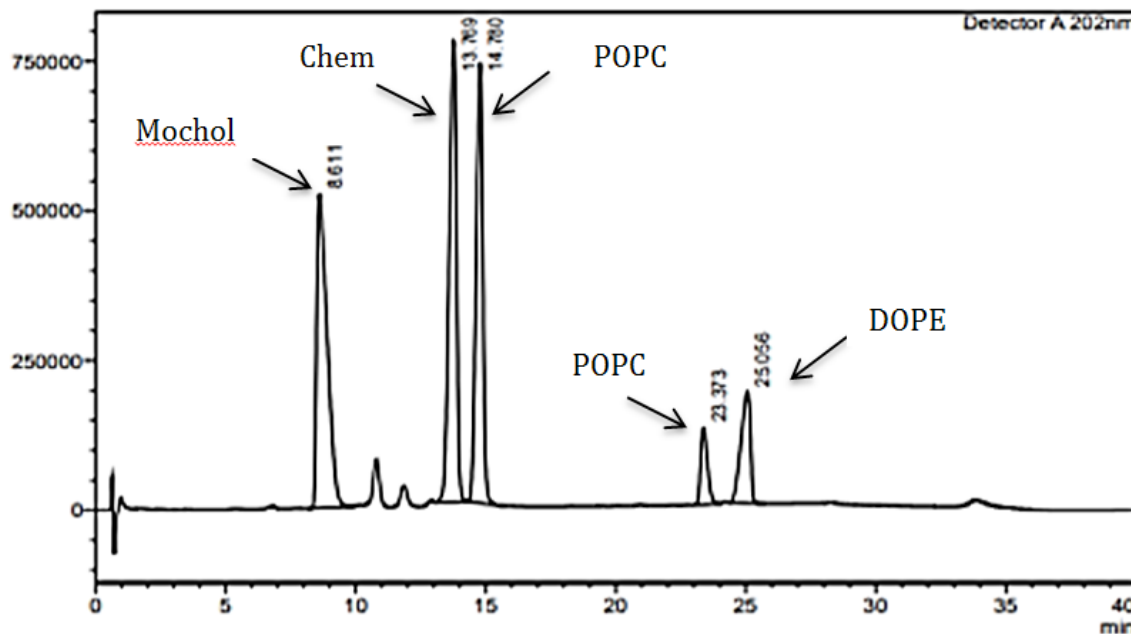
Figure 2. Chromatograms of DOPE, POPC, MoChol, Chems, and Cholesterol at 500 mg/L for each lipid
